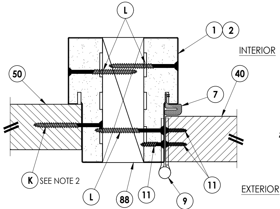
1 6 HORIZONTAL CROSS SECTION Outswing
