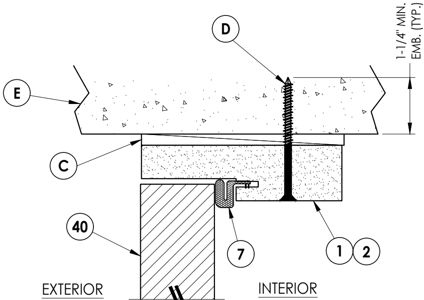
3 8 VERTICAL CROSS SECTION Shown Direct to Masonry
