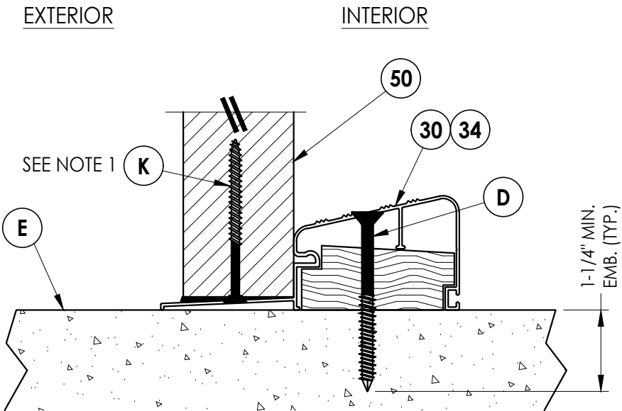
3 10 VERTICAL CROSS SECTION
